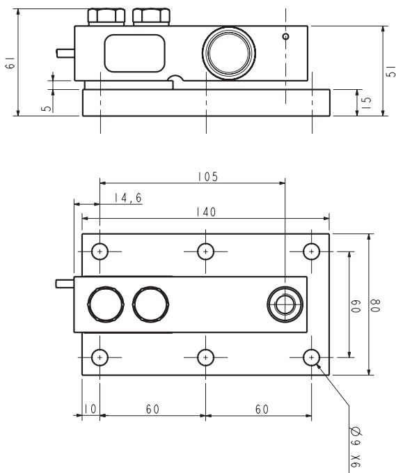
Sockel QUICKFIT-S 2t - Base plate QUICKFIT-S 2t
