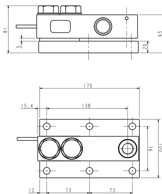
Sockel QUICKFIT-S 5t - Base plate QUICKFIT-S 5t
